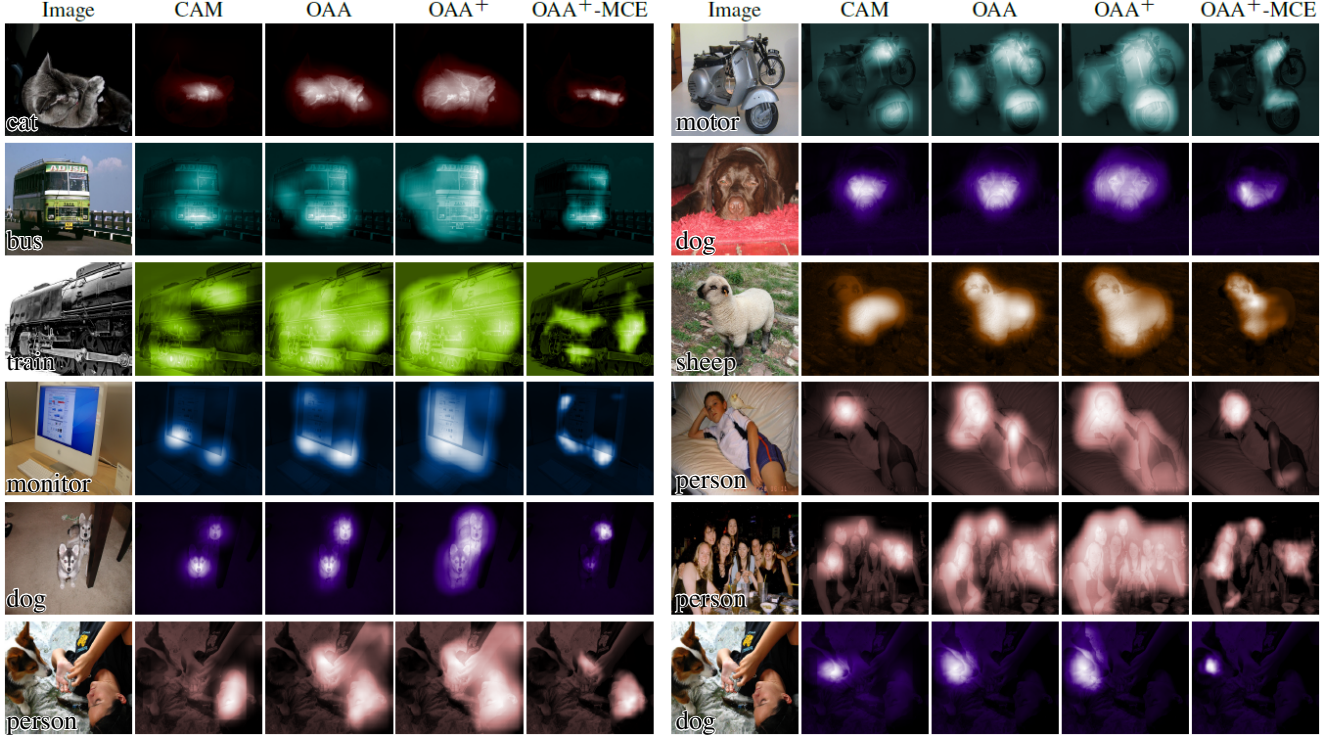
Figure 5. Visual comparisons among different attention maps produced by CAM [49], OAA, OAA^+ and OAA^+-MCE . OAA^+ and OAA^+-MCE denote the integral attention model learned with the proposed hybrid loss in Eq. (9) and the multi-label cross entropy loss in Eq. (6) respectively.
